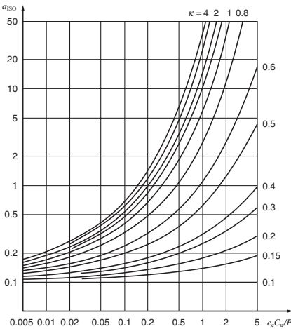
Fig. 1-3 Life modification factor a_{ISO} (Radial roller bearings)
