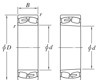
Cylindrical bore Tapered bore
