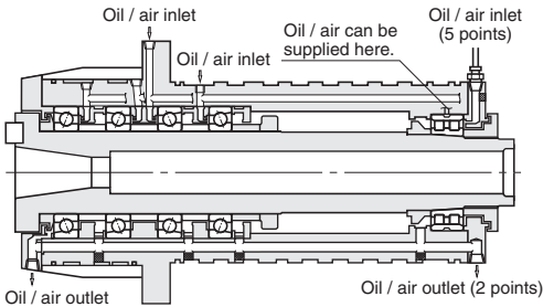
(Example of spindle unit incorporating oil / air lubrication system)
