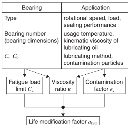
Fig. 1-1 System approach
