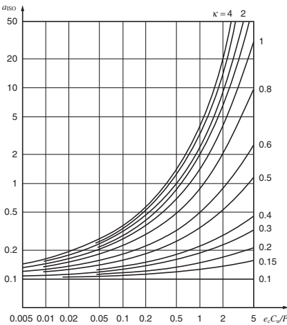
Fig. 1-5 Life modification factor a_{ISO} (Thrust roller bearings)
