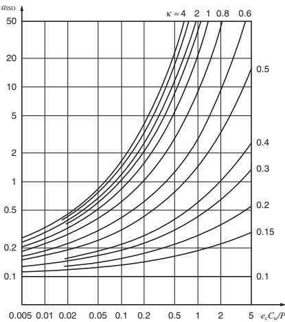
Fig. 1-4 Life modification factor a_{ISO} (Thrust ball bearings)
