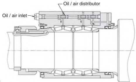
(Example of rolling mill roll neck bearing)
