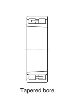
NNU ... K type
