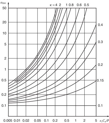
Fig. 1-2 Life modification factor a_{ISO} (Radial ball bearings)
