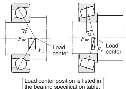
Fig. 1-7 Axial component force
