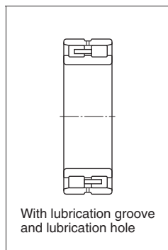
NN ... W type
