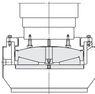
Mounting example of tapered roller thrust bearing for screw down spindle
