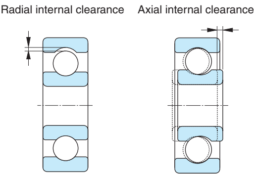
Fig. 6.1 Bearing Internal Clearance
