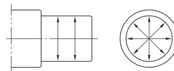
Fig. 11.1 Shaft Diameter Measuring Positions
