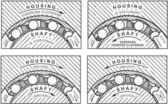
Clearance between the rollers and cup ramps is exaggerated in these drawings. Fig. B3-6. Overrun mode and lock mode
