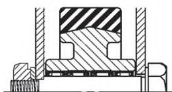
Fig. B3-7. Clutch and bearing arrangement for heavy loads
