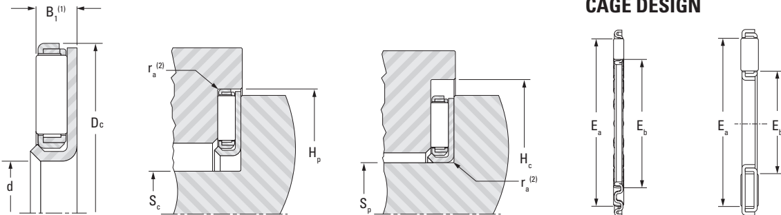
Housing Piloting
