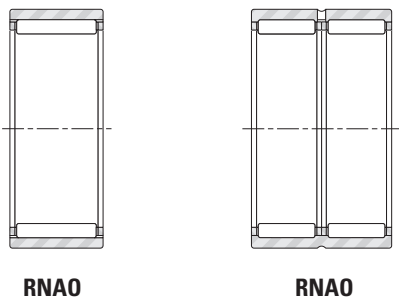
Fig. B4-6. Needle roller bearings without flanges, without inner rings
