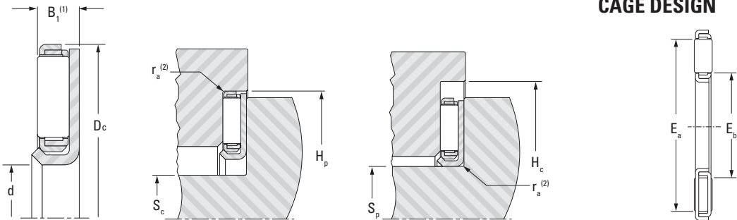
Housing Piloting
