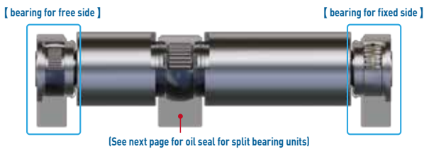
Roll configuration example 2 (pestle-shaped roll)
