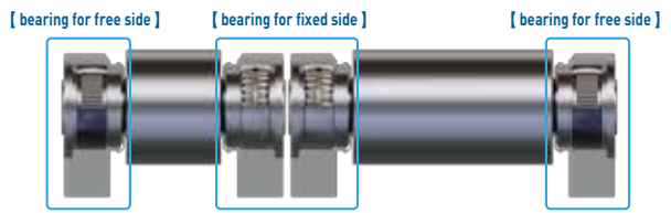
Roll configuration example 1 (single and split rolls)
